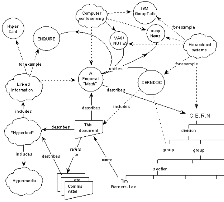
Figure 7 Tim Berners-Lee's flow chart for the Web
