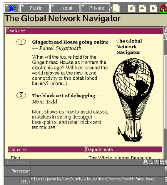
Figure 8 ViolaWWW Screenshot.
